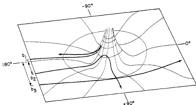
Figure 1. A representation of the potential energy between a fixed target atom and a projectile atom as a function of their internuclear separation. Representative trajectories are shown for cases in which the aiming error or impact parameter b of the projectile is small, medium, and large. The scattering angle in a collision is measured from the original direction of the projectile to the final straight-line portion of its trajectory. Note that the curvature of the trajectory, and hence the scattering angle, is principally determined by the behavior of the projectile near the distance of closest approach to the target.
